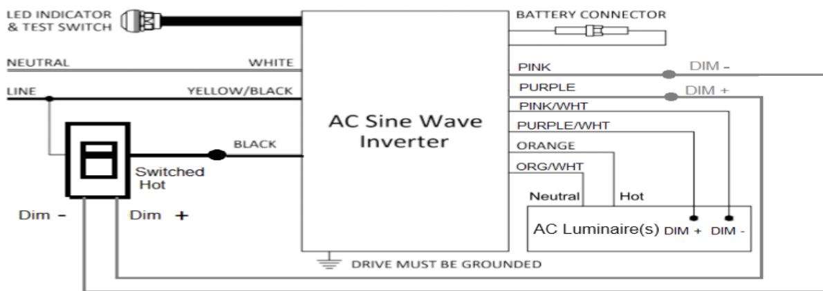
Figure A. Wiring Diagram with 0-10V Dimmer 115W Max. Connected Load ( 23W Emergency)
