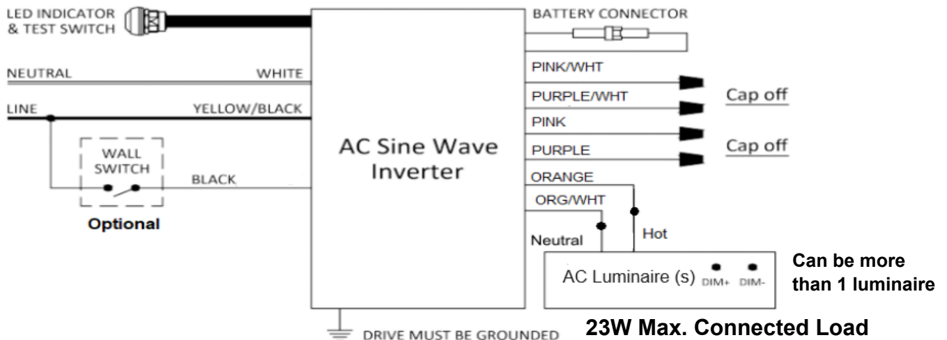
Figure B. Wiring Diagram without 0-10V Dimmer
